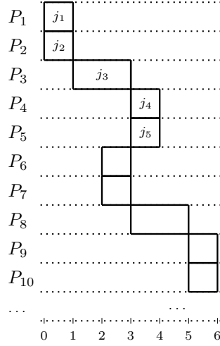
Fig. 4. The idealized schedule S_\infty for the synchronous arrival sequence of the DAG task in Figure 2 (only a prefix of the schedule is shown).
