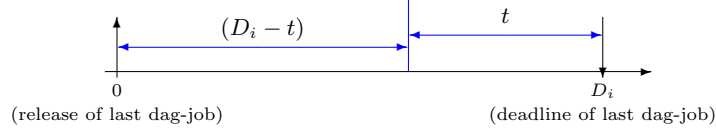
Fig. 8. Computing \text{work}(\tau_i, 70, 1) for the task \tau_i of Figure 9.
