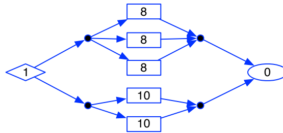
Fig. 9. The DAG \mathcal{G}_i of an example conditional dag-task \tau_i . For this task, D_i = 15 and T_i = 20 . Note that \text{len}(\mathcal{G}_i) = 11 and corresponds to taking the lower branch of the conditional, while \text{vol}(\mathcal{G}_i) = 25 and corresponds to taking the upper branch.
